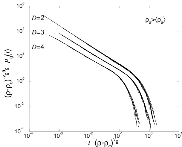
Fig. 3. Scaling analysis of the global persistence distribution P_g^>(t) for various dimensions. With increasing dimensions the slope of the curves ( i.e. the exponent \theta_g ) decreases slightly. The curves of the three- and four-dimensional system are shifted in the lower-left direction. The corresponding data-collapses for P_g^<(t) are of similar accuracy (not shown).
