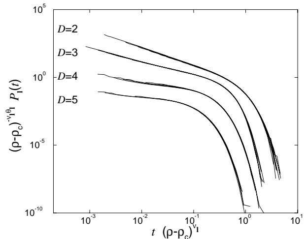
Fig. 4. Scaling analysis of the local persistence distribution P_1(t) for various dimensions. With increasing dimensions the slope of the curves ( i.e. the exponent \theta_1 ) decreases. For D = 3, 4, 5 the corresponding curves are shifted in the lower-left direction.
